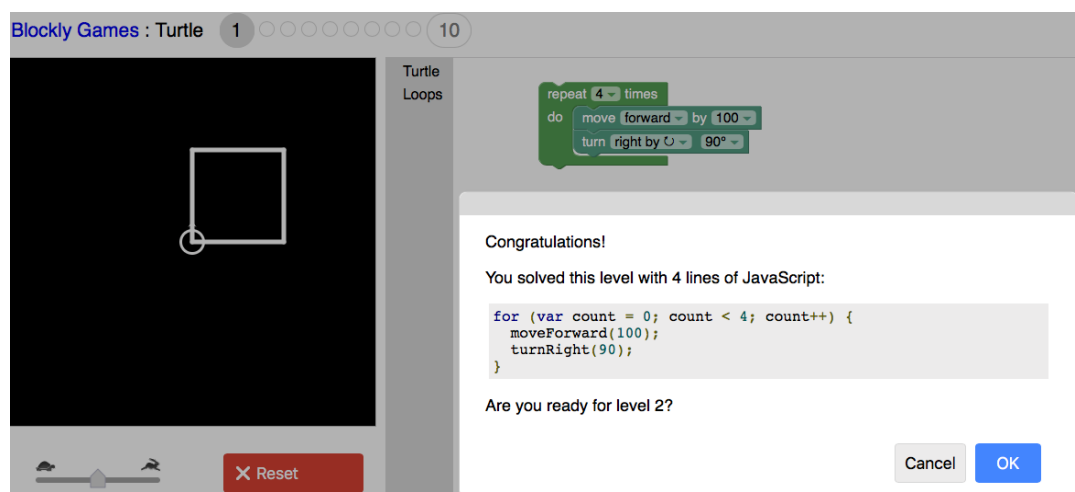
Figure 97: Example of Blockly code using variables
