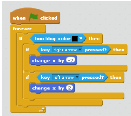
Figure 57: Code for moving away from an edge if right or left arrows were pressed
